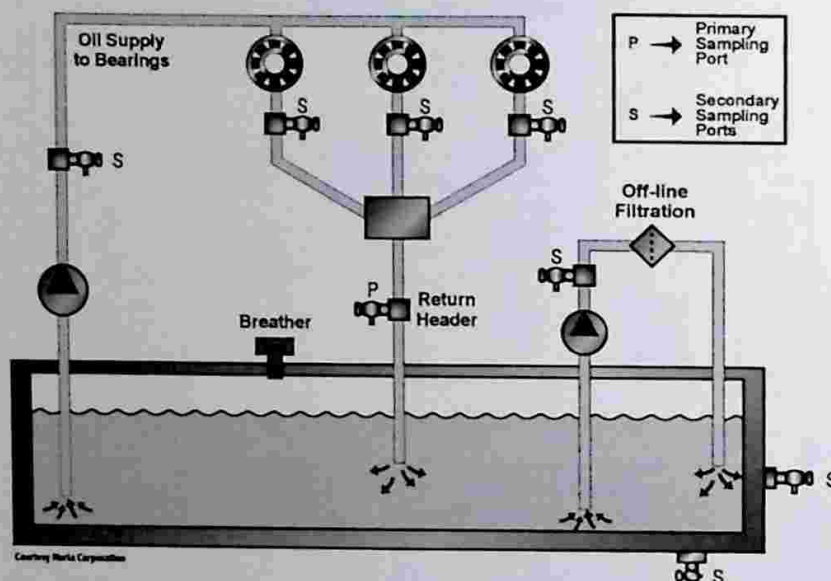
Figure 15.4a Optimum Sampling Point in Circulating Oil Systems
