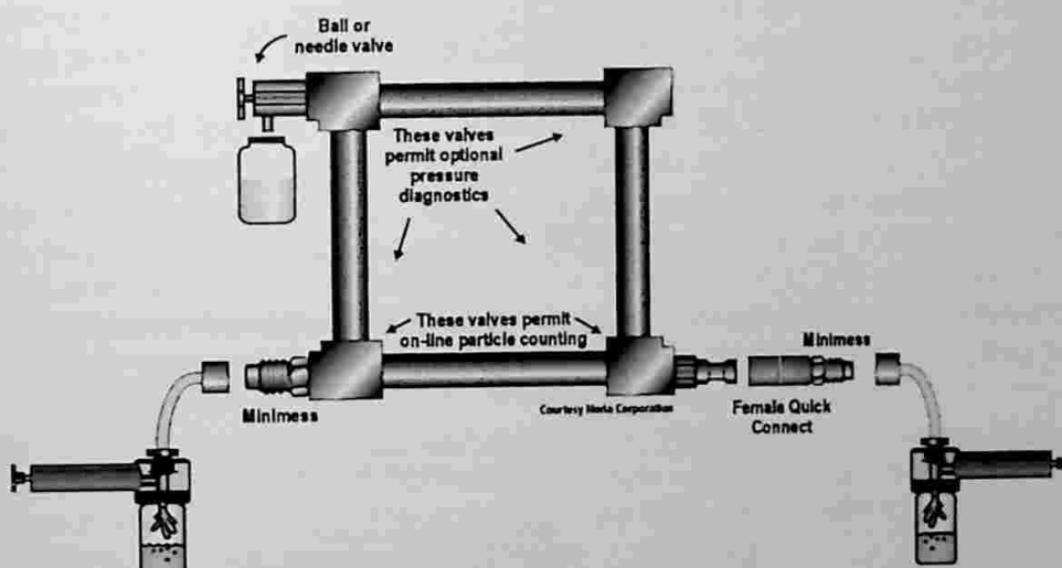
Figure 15.4d Vacuum Pump Assists the Oil Flow of High Viscosity Lubricants
