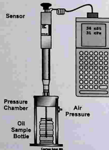
Figure 15.10 An Absolute Viscometer Designed for Plant-Level Use
