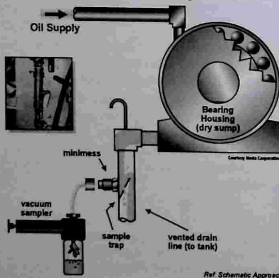
Figure 15.4b Options for Sampling Low Pressure Return Lines
