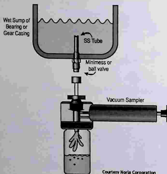
Figure 15.5 Sampling for Splash, Slinger Ring, and Flood-Lubricated Components
