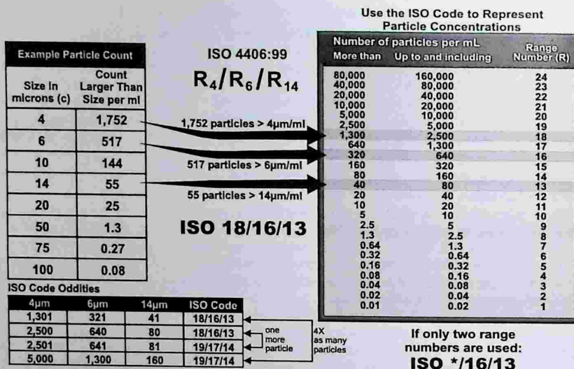
Figure 15.13 ISO 4406 Two-Range Number System for Representing Particle Counts in Oils
