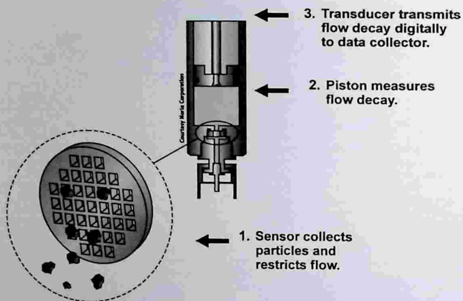
Figure 15.16 Pore Blockage-Type Particle Counters Can Discriminate Between Hard Particles and Other Impurities
