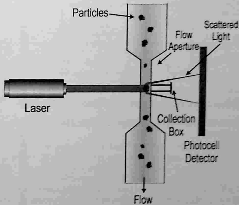
Figure 15.15 Particle Counters Using Laser or White Light Can Count Particles Across a Wide Range of Sizes
