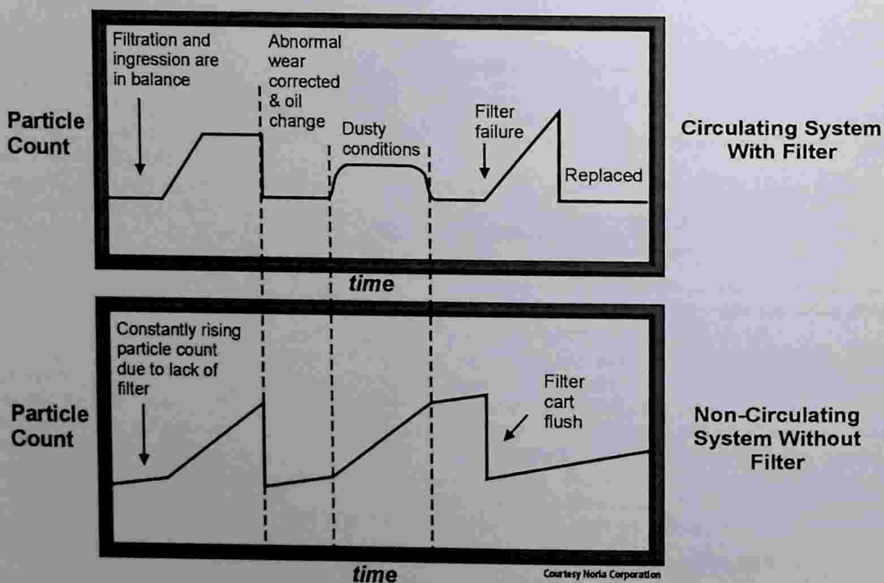
Figure 15.17 Particle Count Trends Vary Depending on the Machine Application and the Presence of an Onboard Filter
