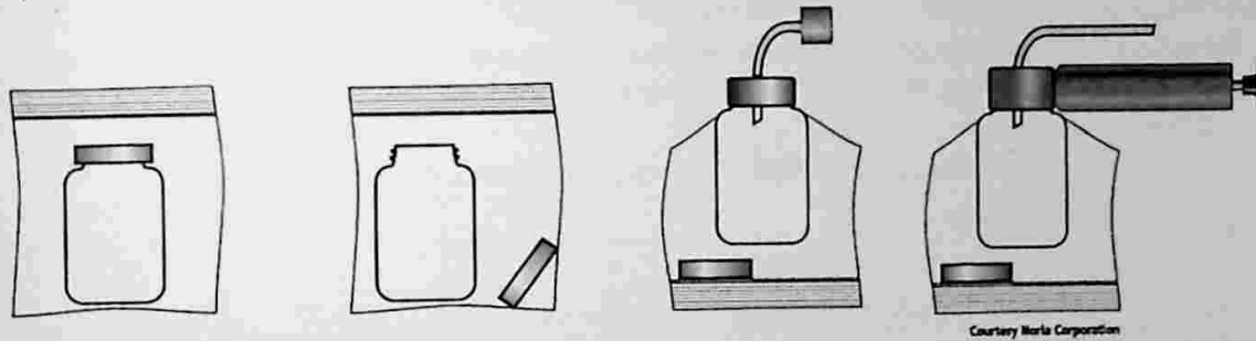
Figure 15.6b Clean Oil Sampling Using Zip-Lock Bags with Sampling Hardware
