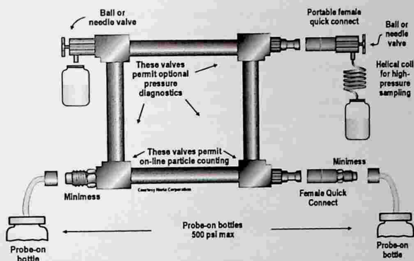
Figure 15.4c Options for Sampling Pressurized Fluid Lines
