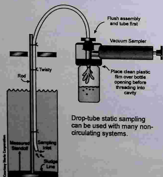
Figure 15.6a Using Drop-Tube Vacuum Samplers for Static Sampling
