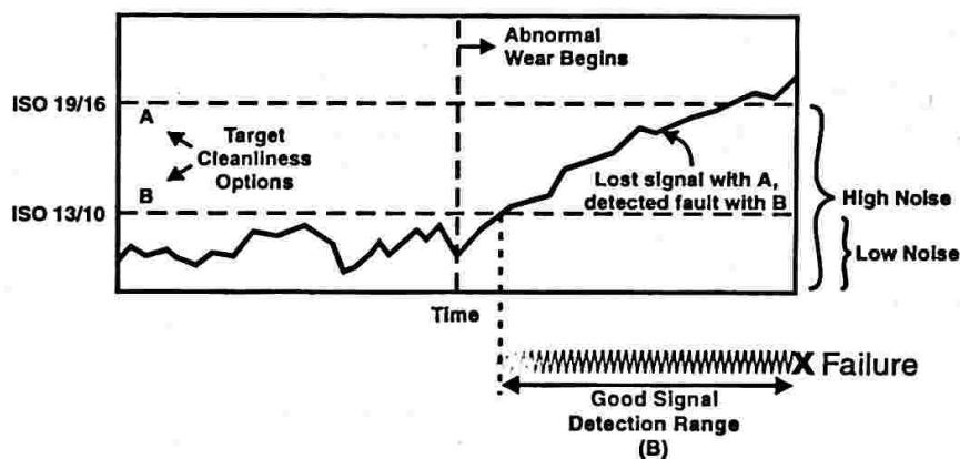
Figure 7 Clean Fluids Help Provide Improved Fault Detection Sensitivity
