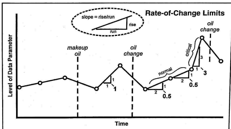
Figure 5 Using Rate-Of-Change Limits (rise/run) Must Be Calculated For The Trending Data Parameter
