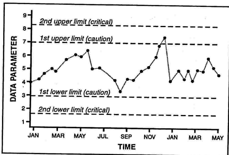
Figure 1 Illustration of Upper and Lower Oil Analysis Limits
