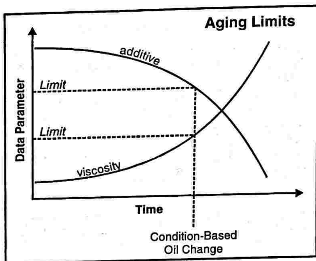
Figure 3 Aging-Limits Are Keyed To Degrading Additive And Base-Stock Properties
